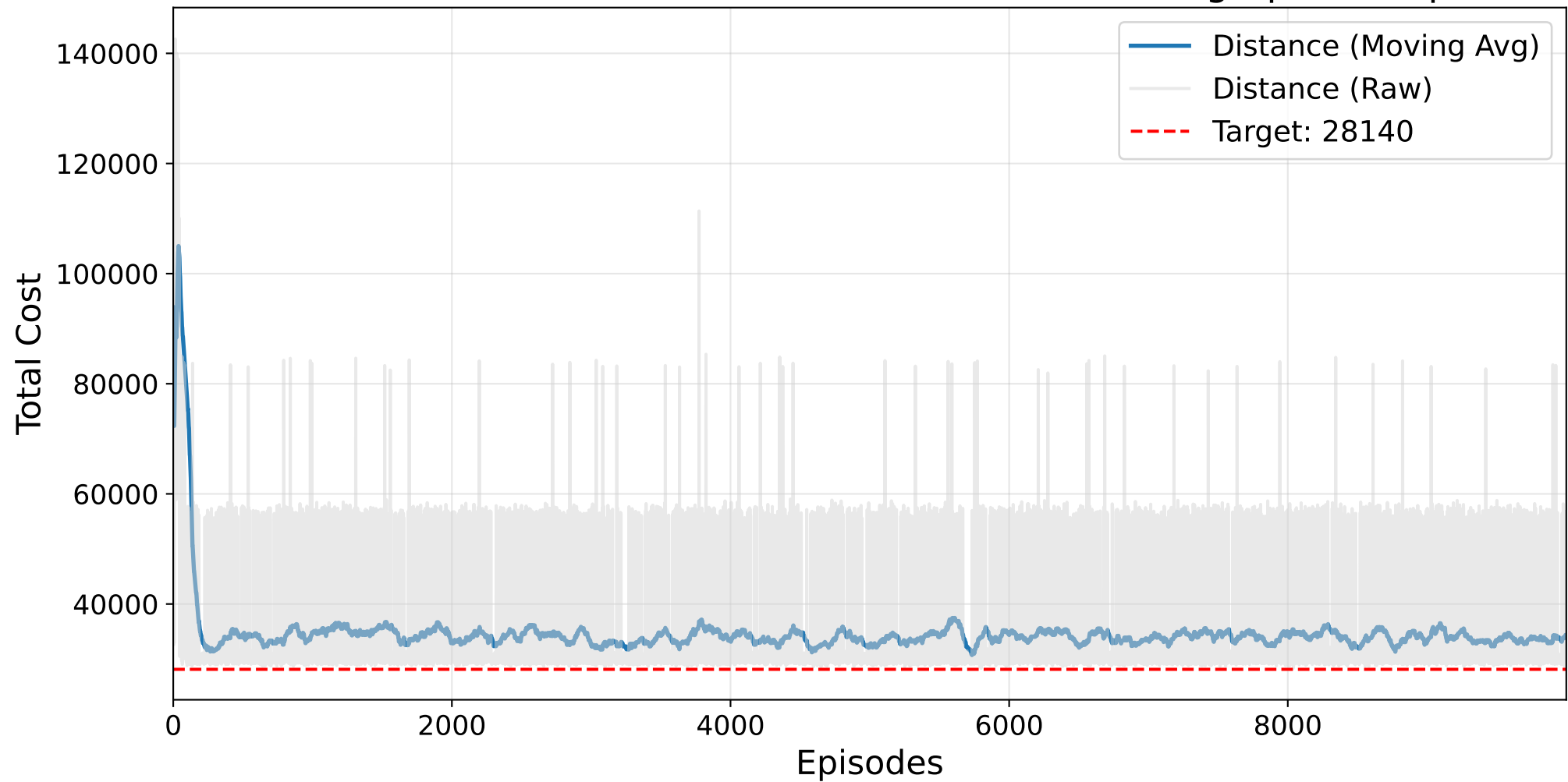
Final HYPERBAND GP Masked AutoRL-SOP Training - p43.1.sop
